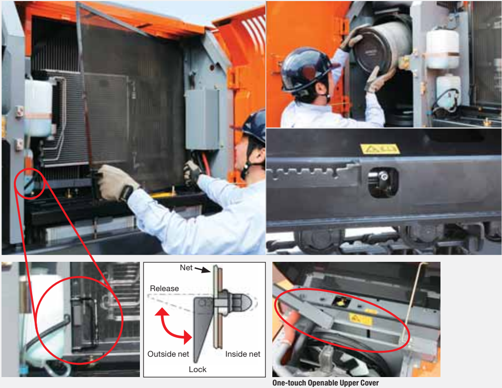
One-touch Openable Upper Cover
